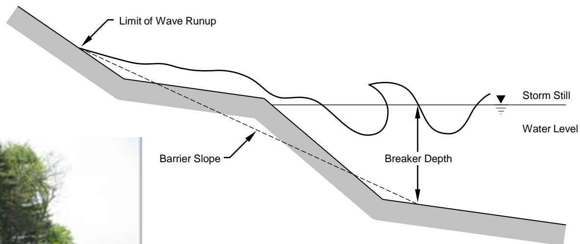
Figure D.3.5-5. Wave Runup Sketch
